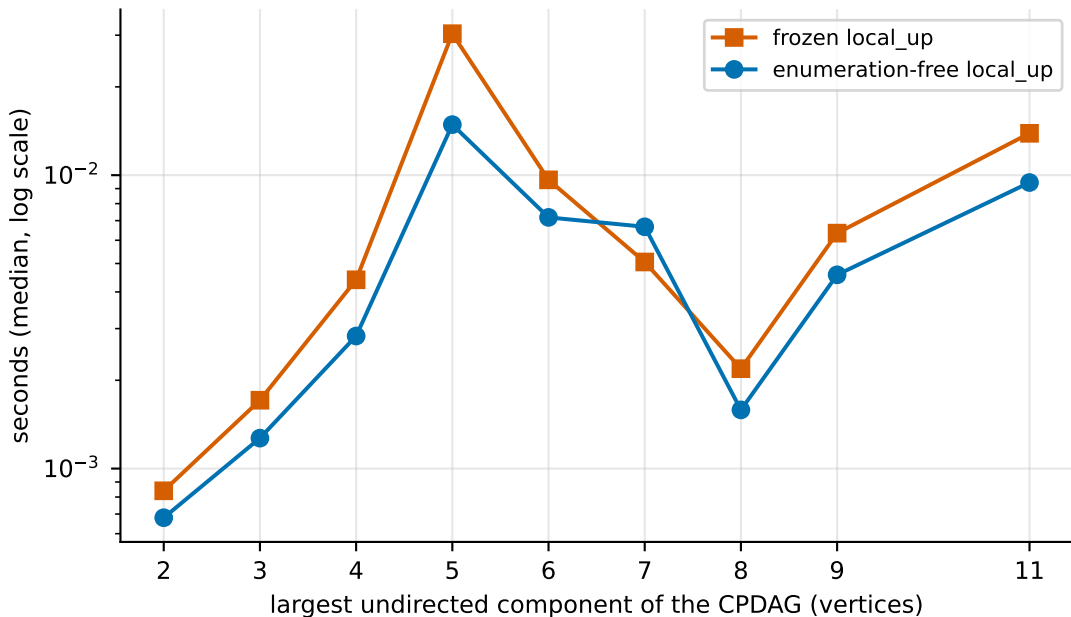
Cost against component size, not n — the axis that matters
