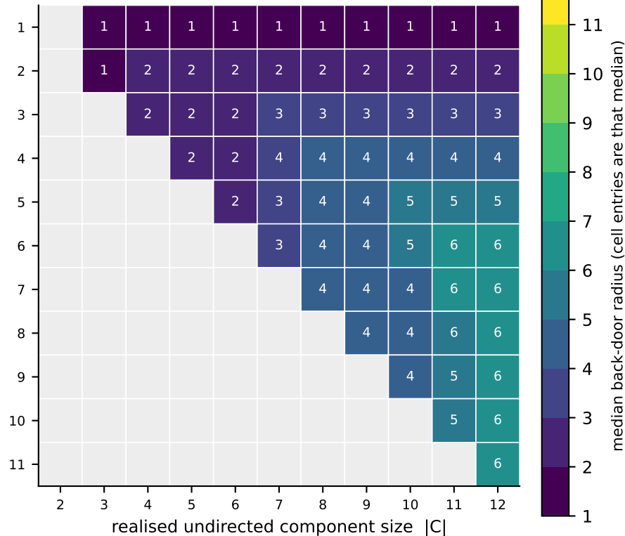
coverage 0.5 — |K_{G0}| now caps r , so rows bend
