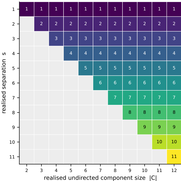
coverage 1.0 — diagonal in s , flat in |component|
