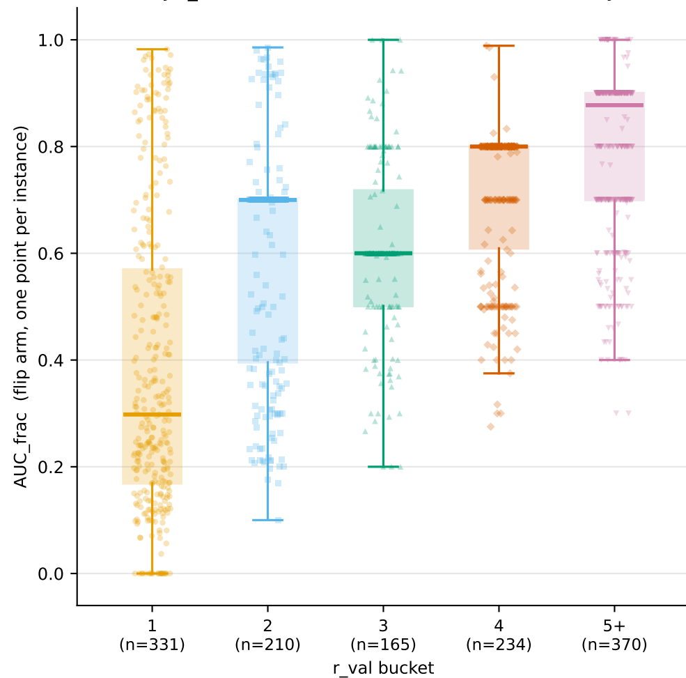
By r_val bucket: rises overall, not monotonically
