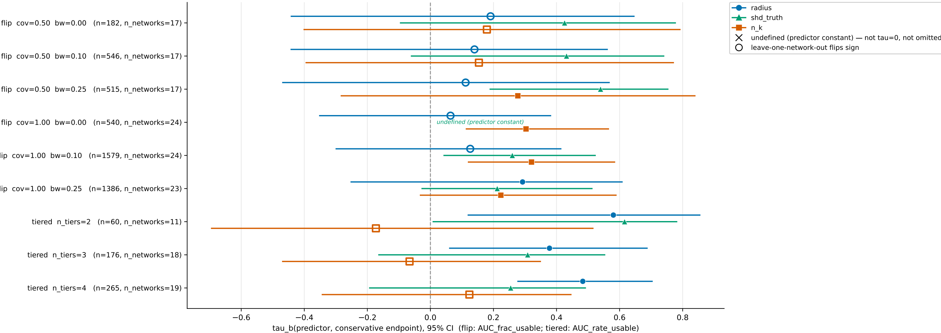
Primary strata: tau_b by predictor, with LOO-network sensitivity flagged
