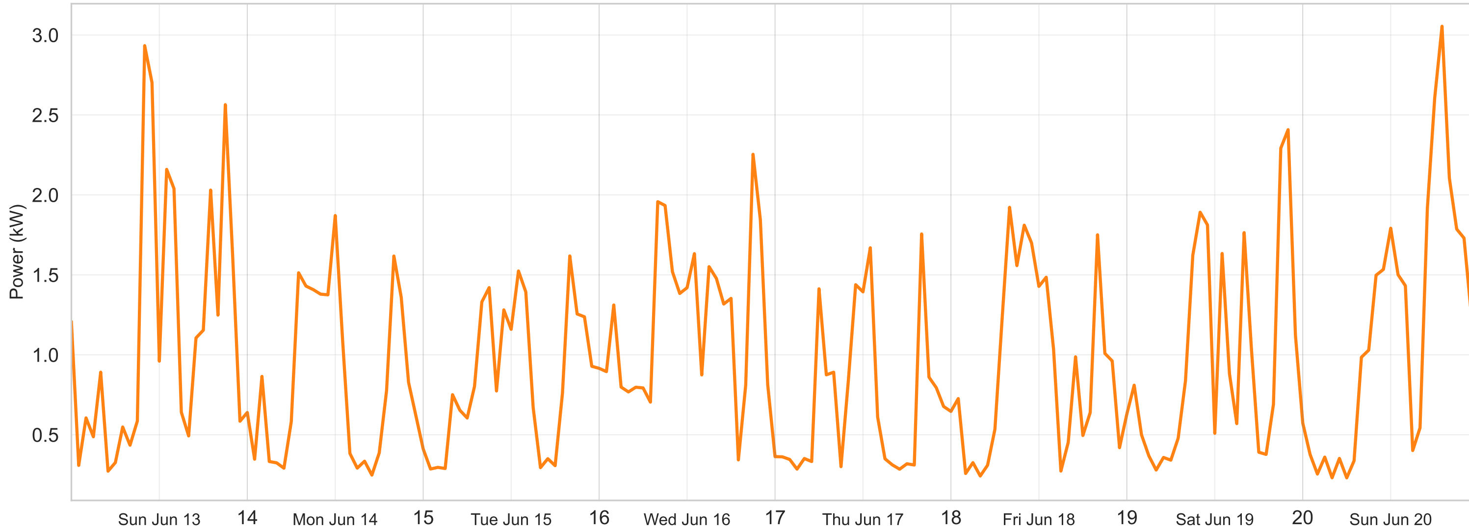
One Week of Electricity Consumption – Typical Week (Jun 13–20, 2010)
