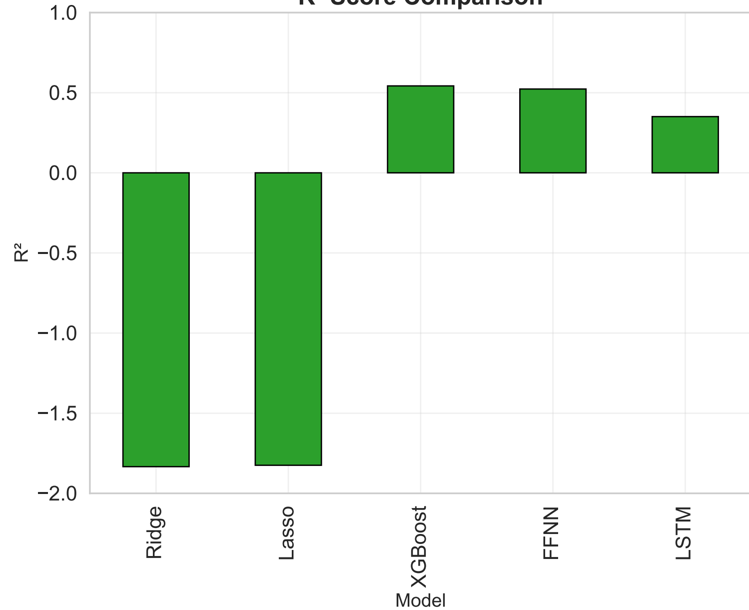
R 2 Score Comparison
