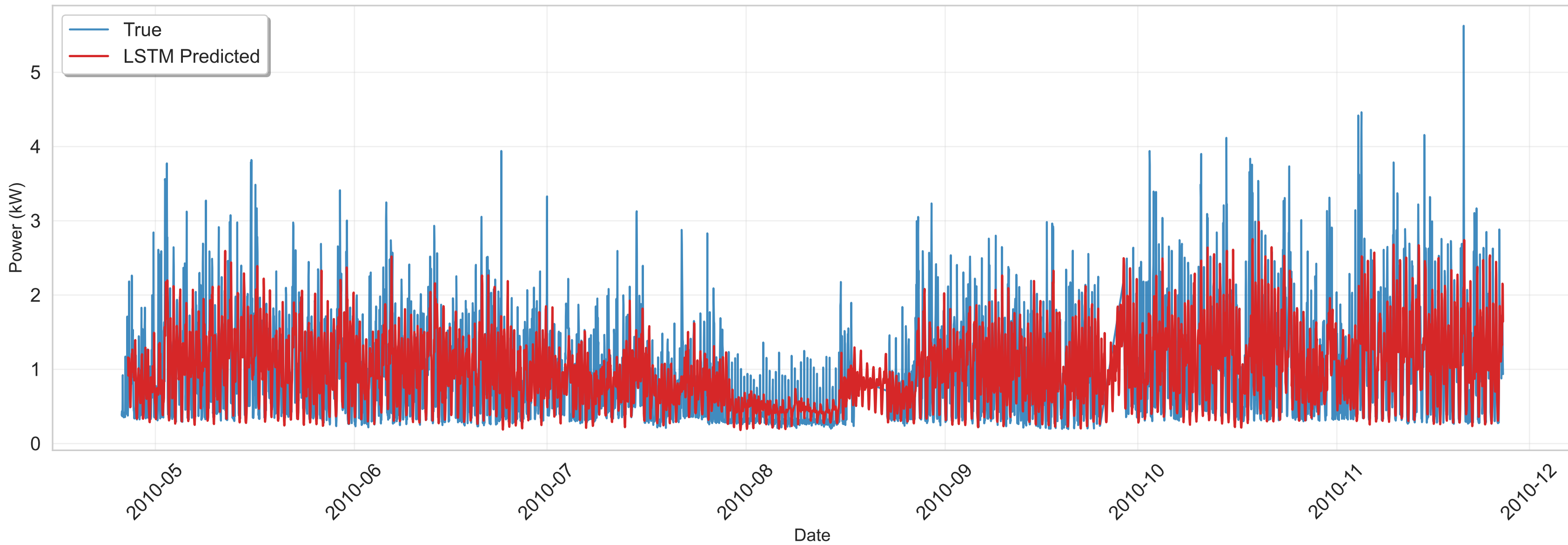
Full Test Period Forecast – LSTM
