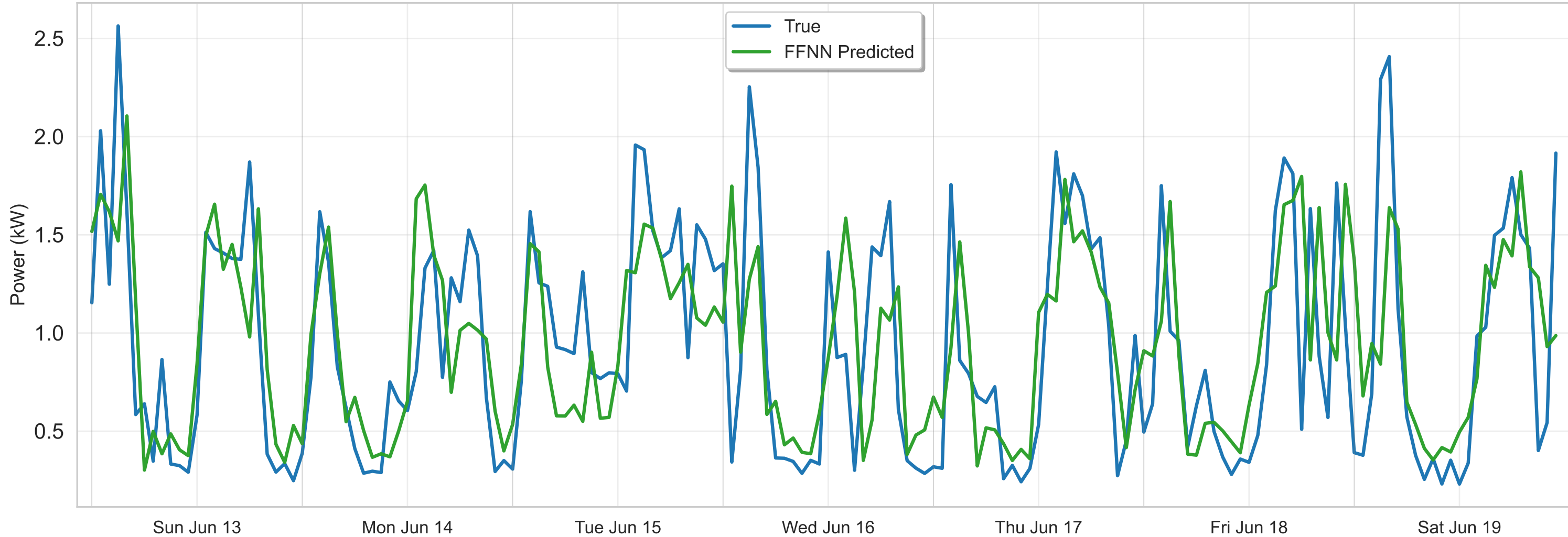
One Week Forecast – FFNN Typical Week (Jun 13 – Jun 20, 2010)
