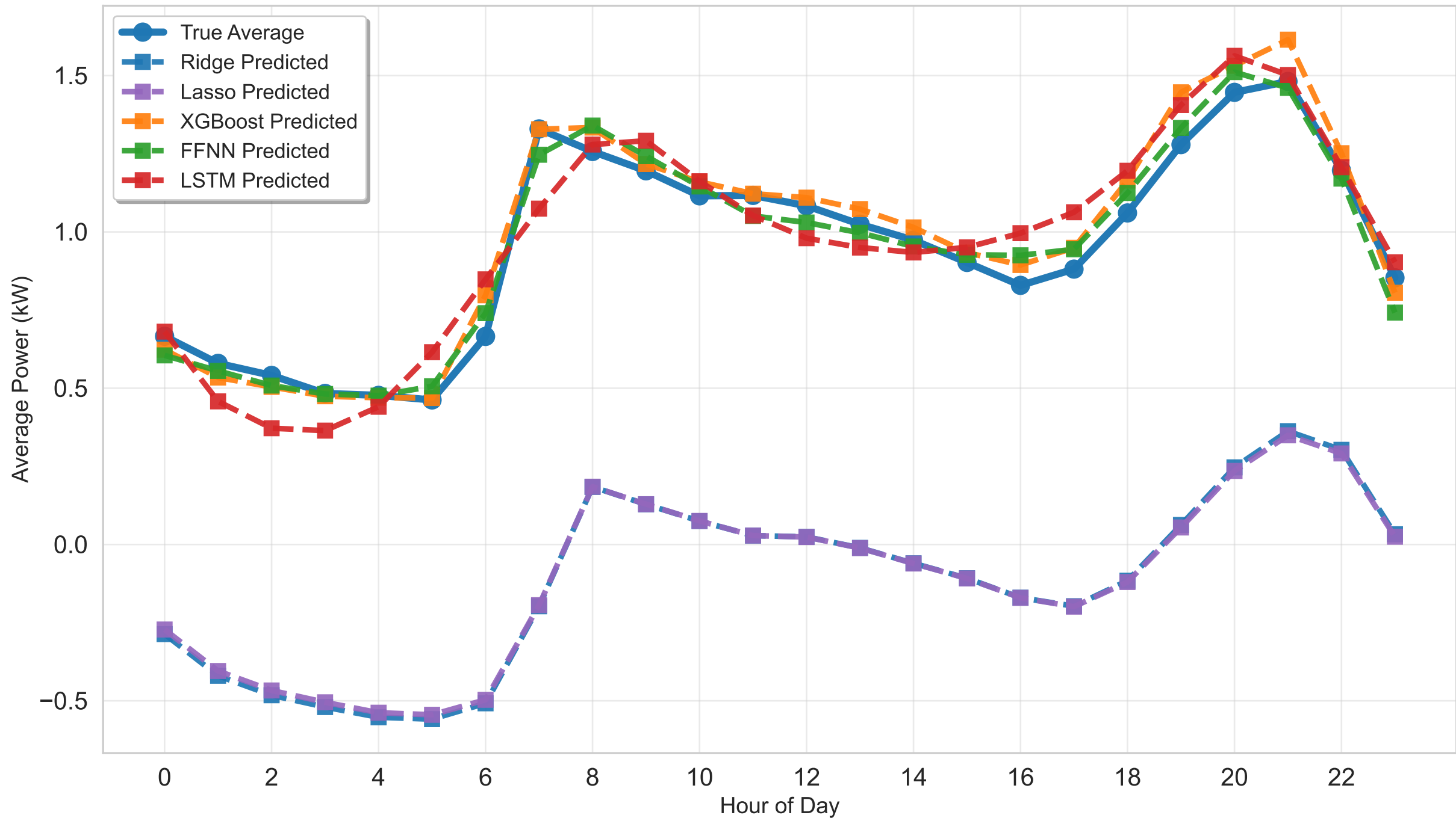
Average Daily Consumption Pattern – All Models
