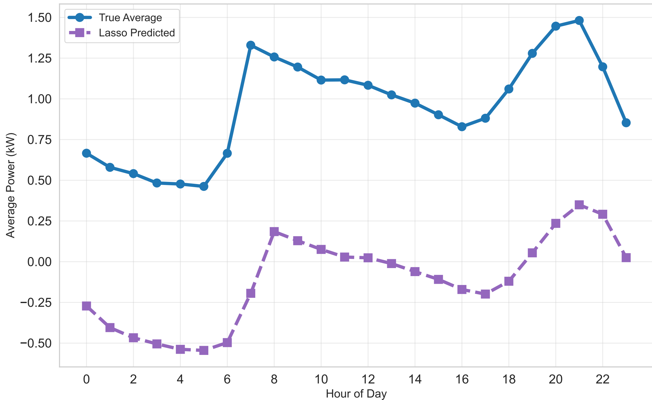
Average Daily Pattern – Lasso
