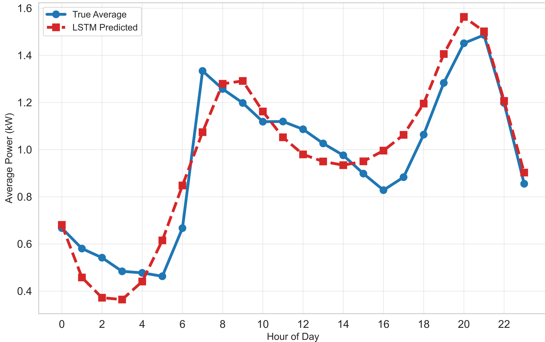
Average Daily Pattern – LSTM
