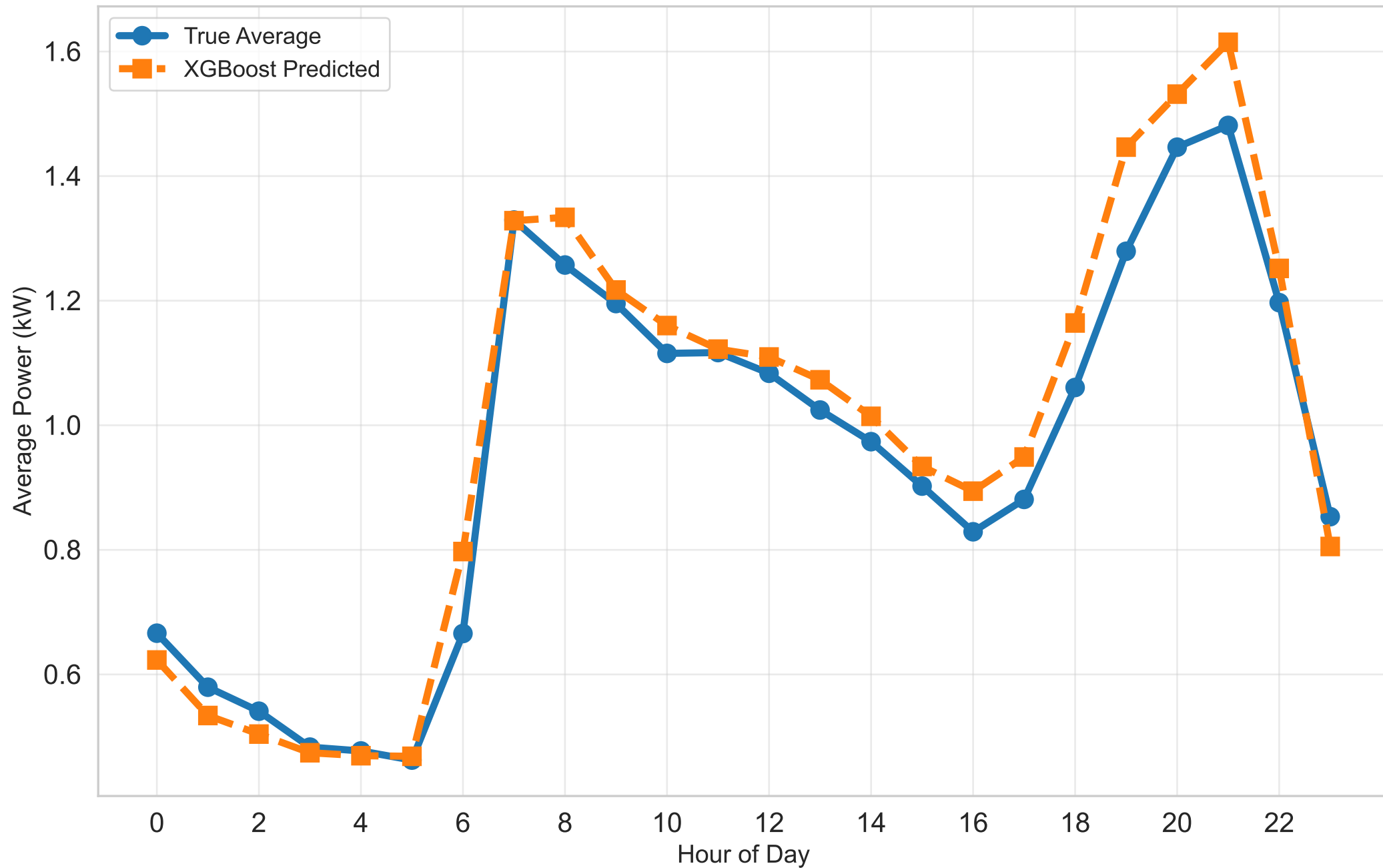
Average Daily Pattern – XGBoost
