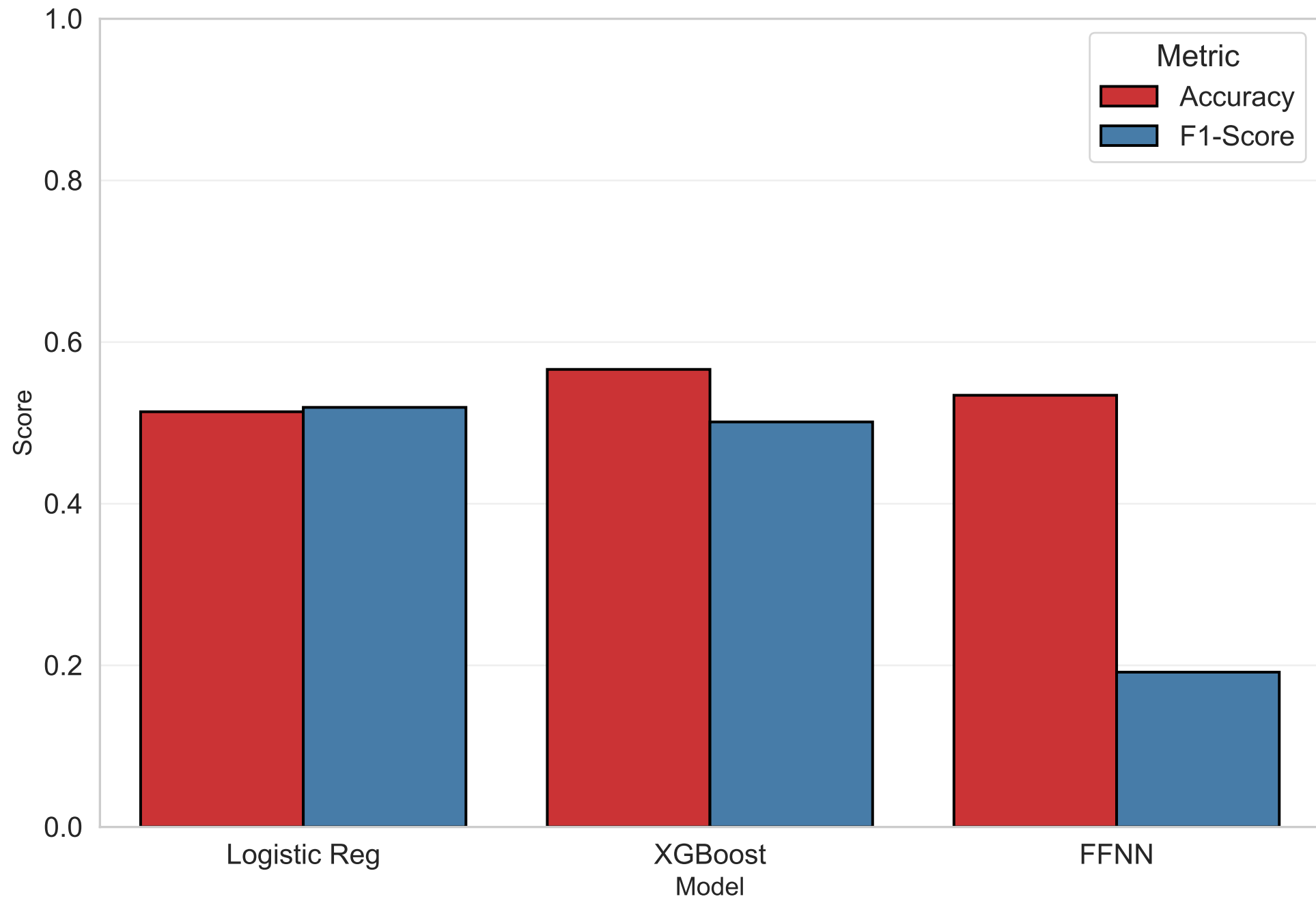
Classification Performance Comparison
