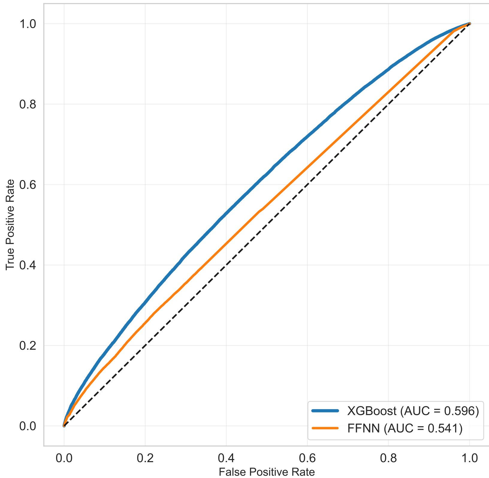
ROC Curve – Trade Growth Classification
