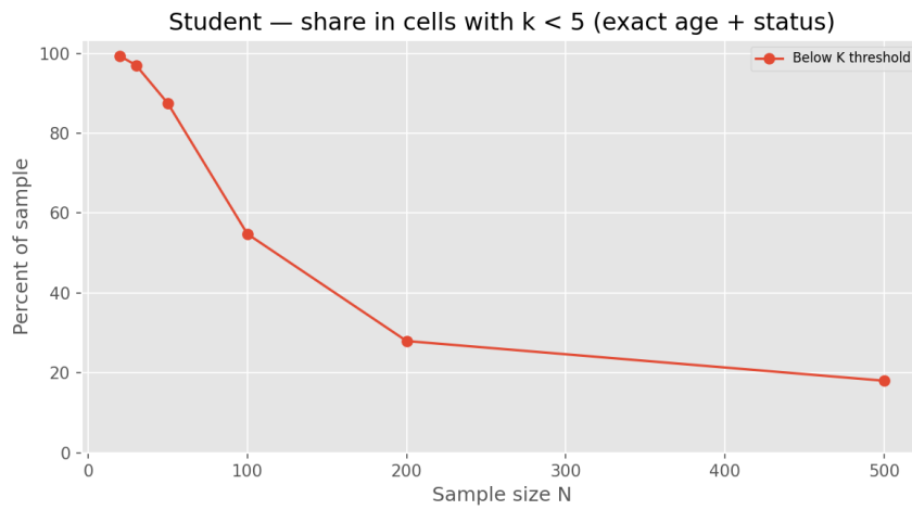
Figure 2: Student cohort: share of participants in equivalence classes smaller than the publication threshold K = 5 .
