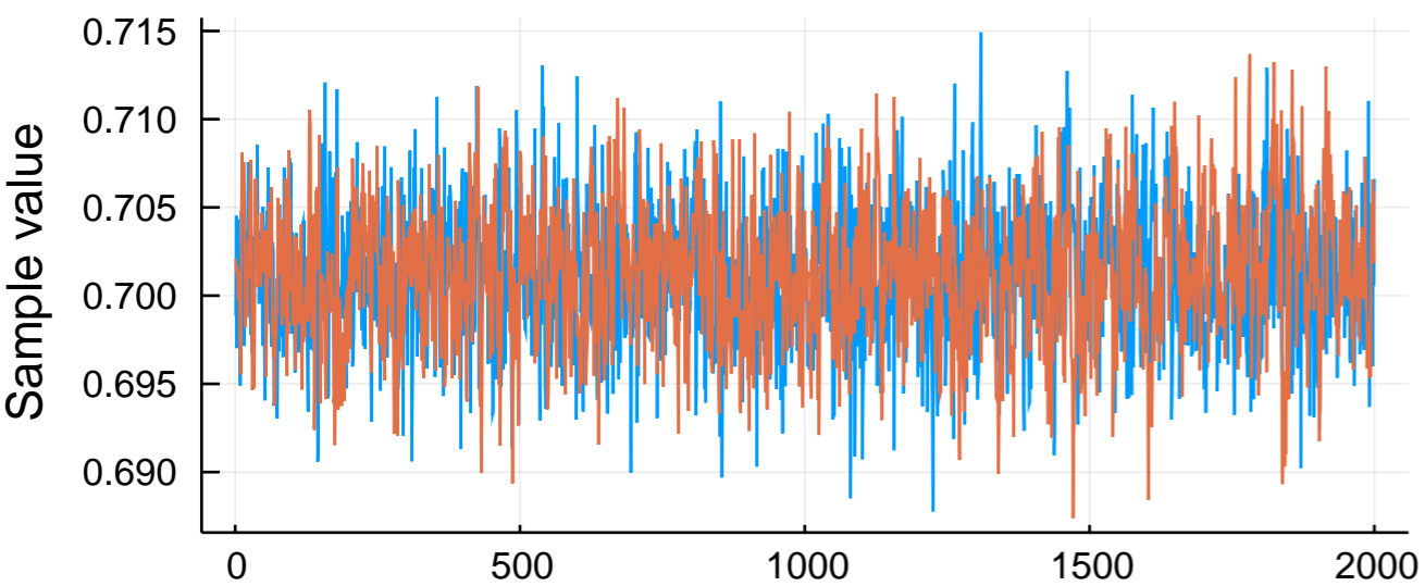
Iteration rho
