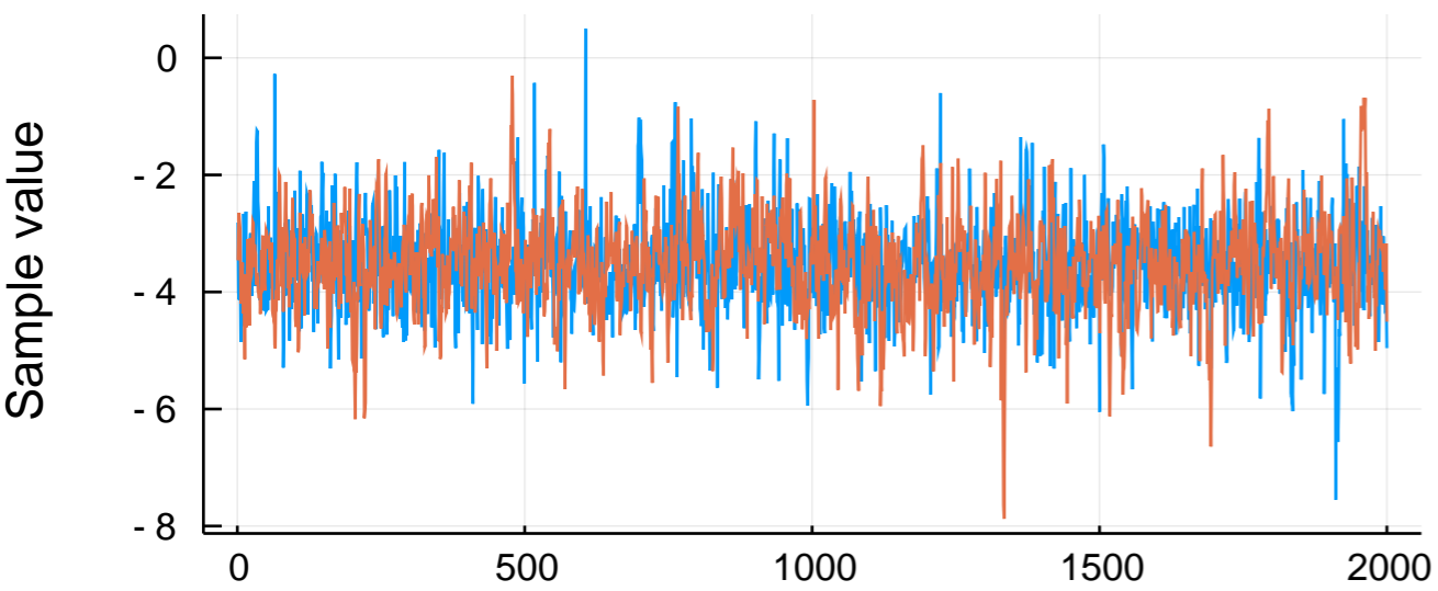
Iteration muh.2
