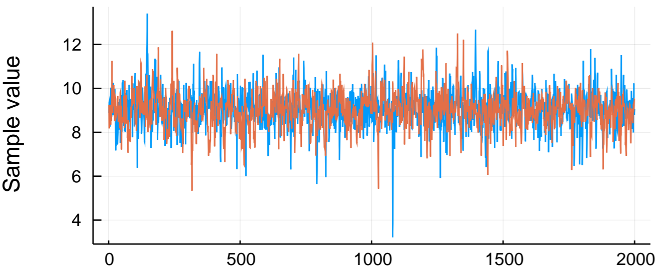
Iteration rho
