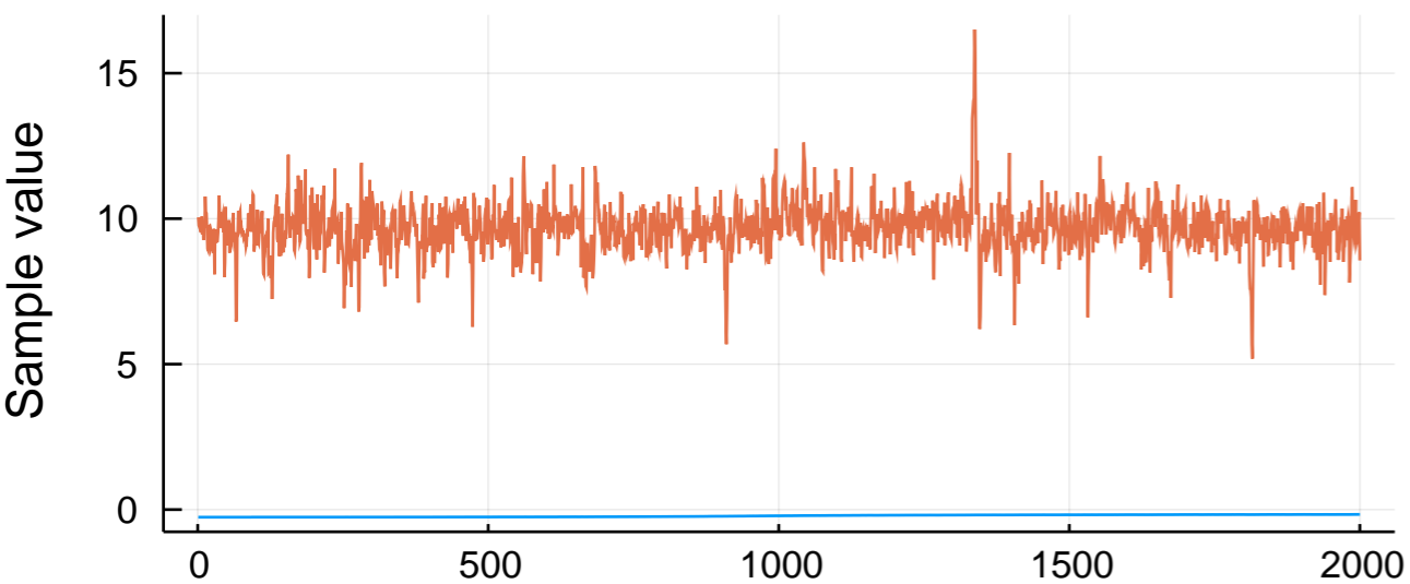
Iteration rho
