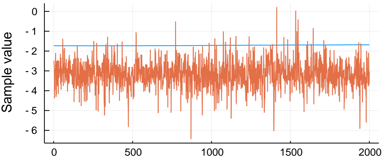
Iteration muh.2
