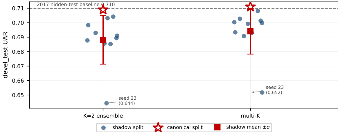
Shadow-split robustness: canonical is one partition in a distribution
