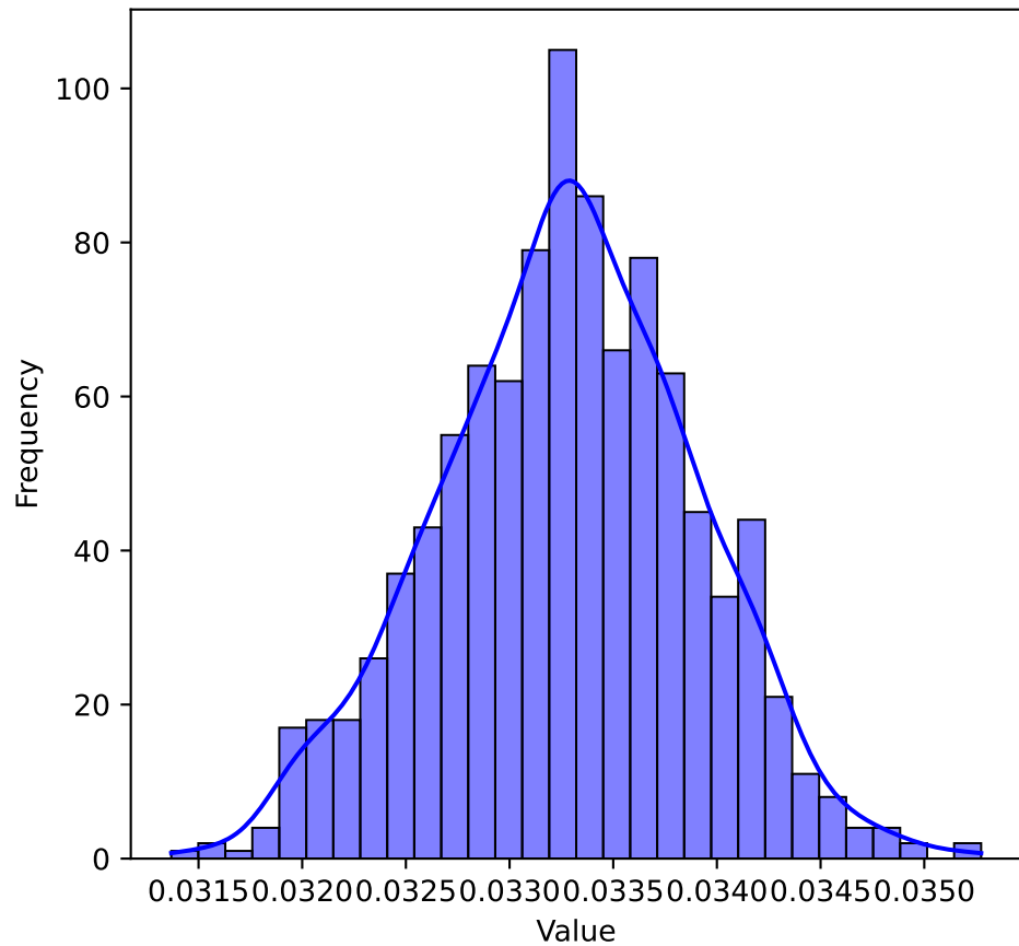
Beta Distribution
