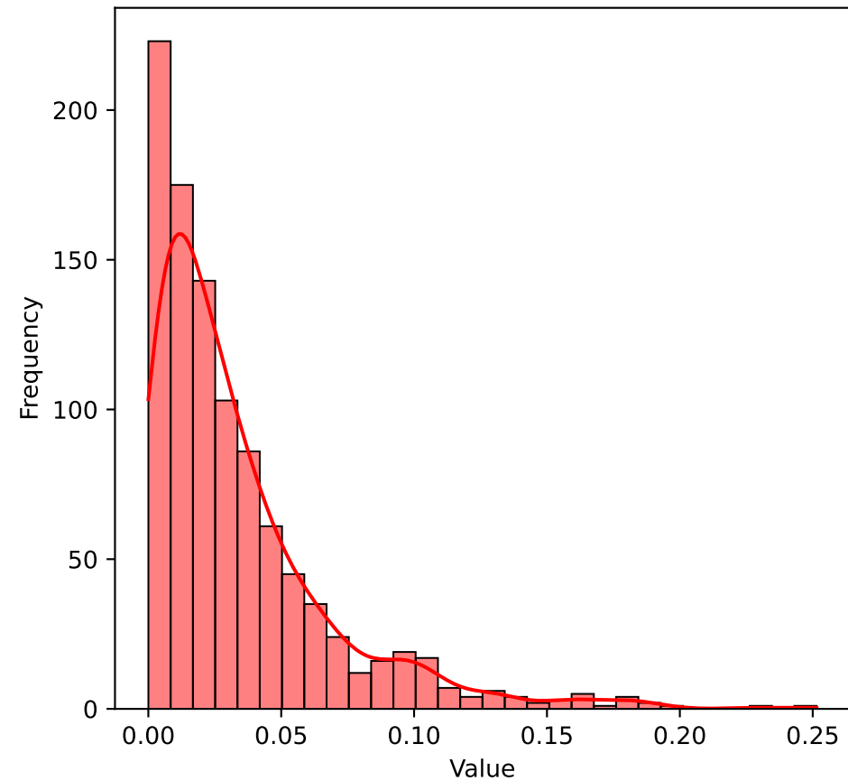
Exponential Distribution
