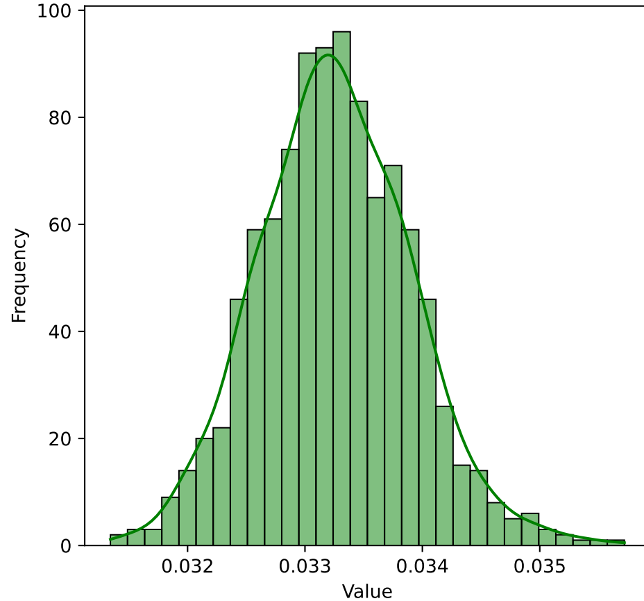
Log-normal Distribution
