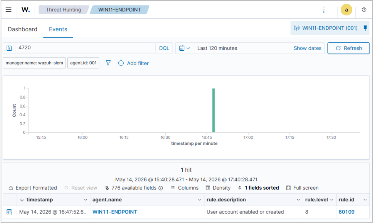
Figure 6. Wazuh Threat Hunting alert overview for user account creation.
