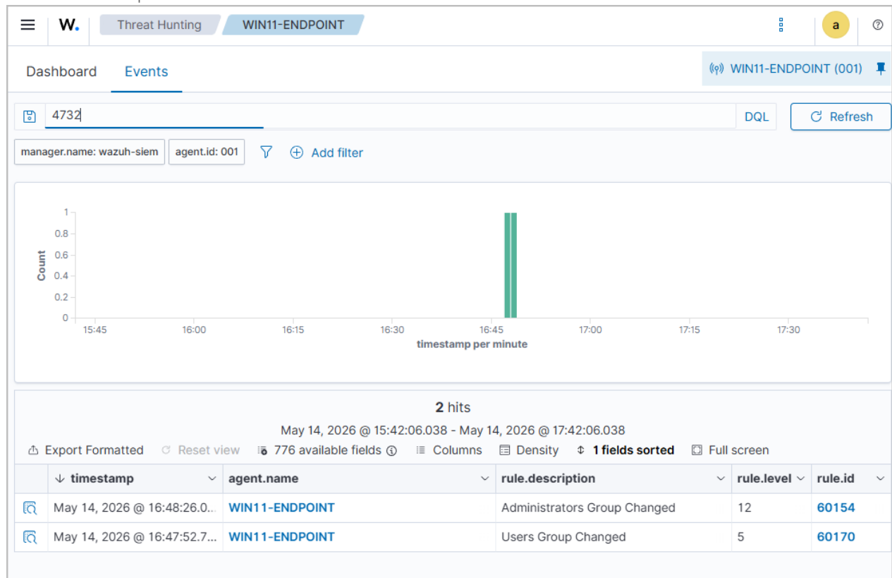
Figure 8. Wazuh Threat Hunting alert overview for Administrators Group Changed.
