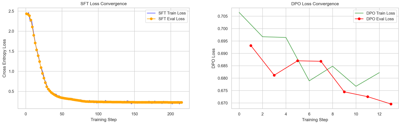
Figure 2. Preliminary training loss curves for Supervised Fine-Tuning (left) and Direct Preference Optimization (right).
