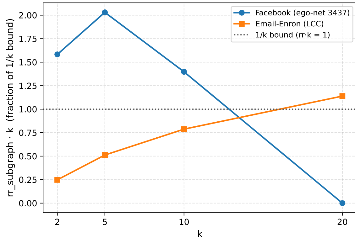
(A) Fraction of 1/k bound — above 1 violates the bound (B1, d=1 )
