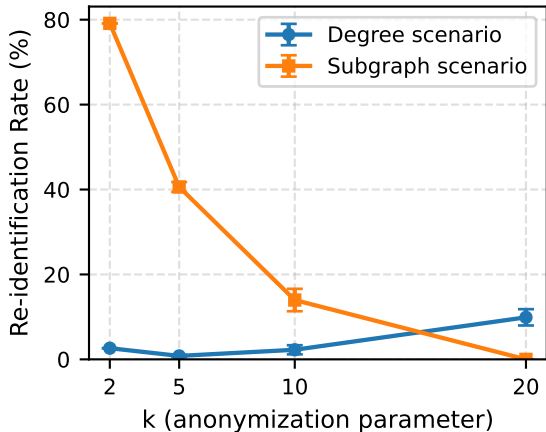
Privacy ( \downarrow better)
