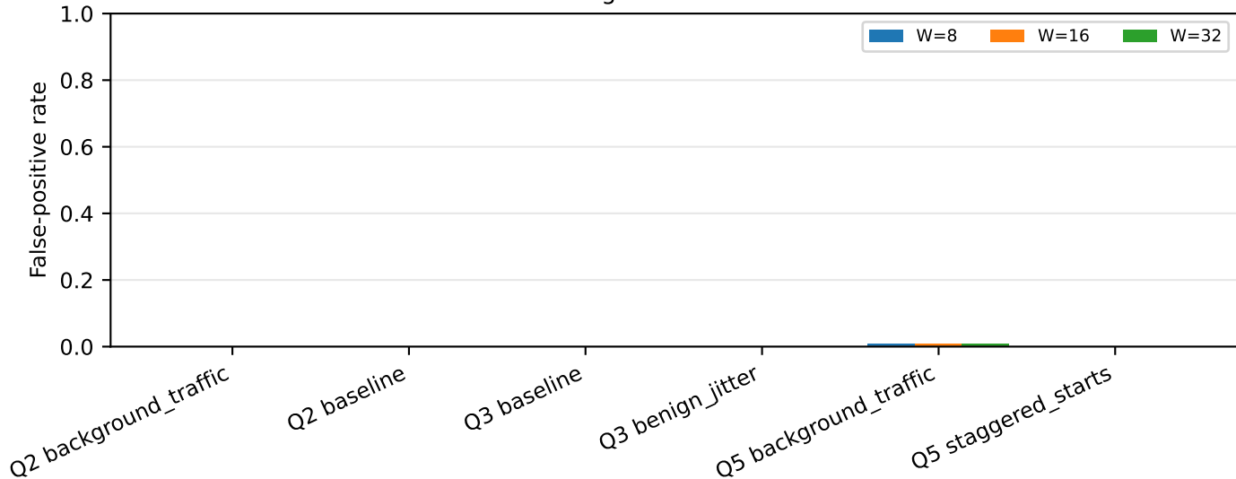
Negative controls
