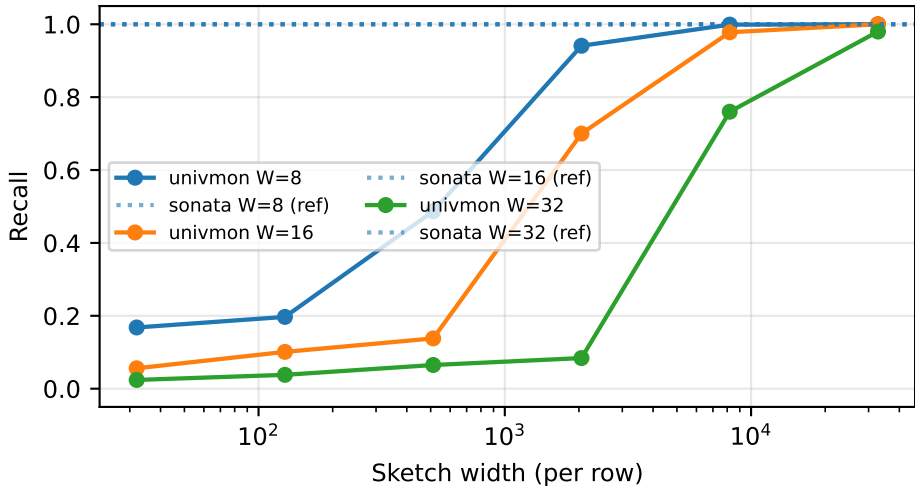
UnivMon Q2 recall vs sketch budget
