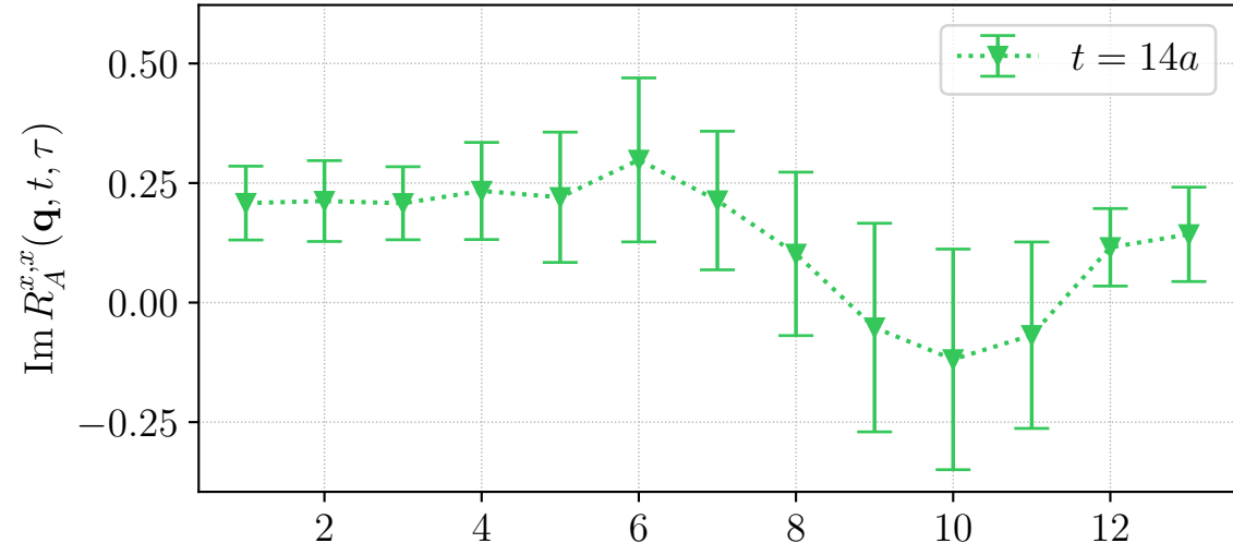
H106, LHP, source id = 1, \mathbf{q} \sim (-1, 2, 1)^\top
