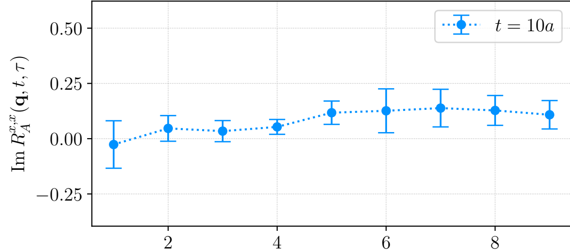
H106, LHP, source id = 0, \mathbf{q} \sim (-1, 2, 1)^\top
