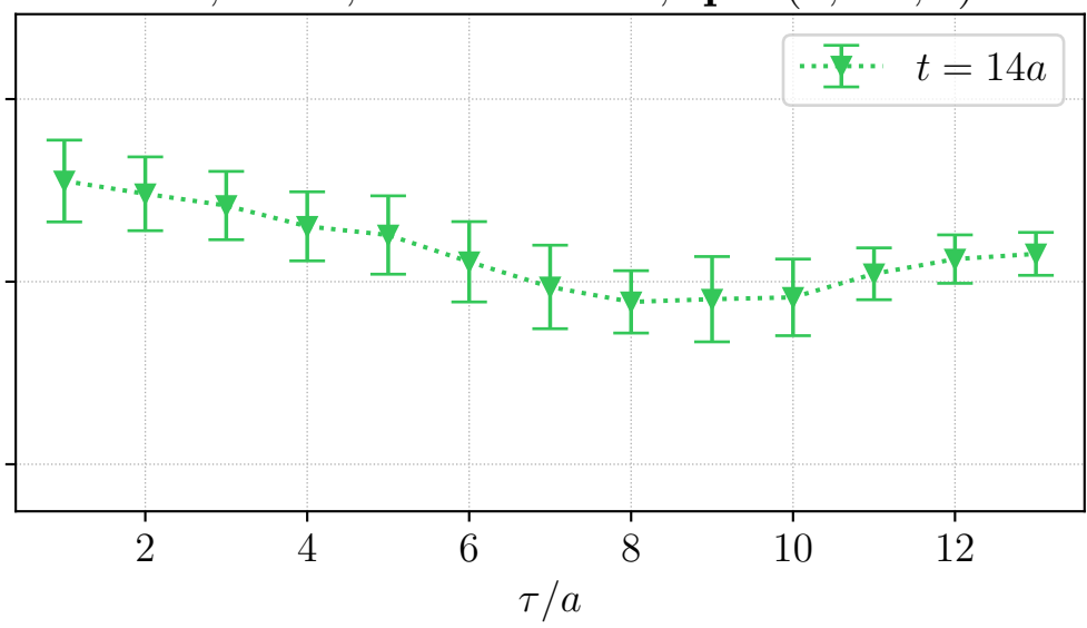
H106, REG, source id = 1, \mathbf{q} \sim (0, -1, 2)^\top
