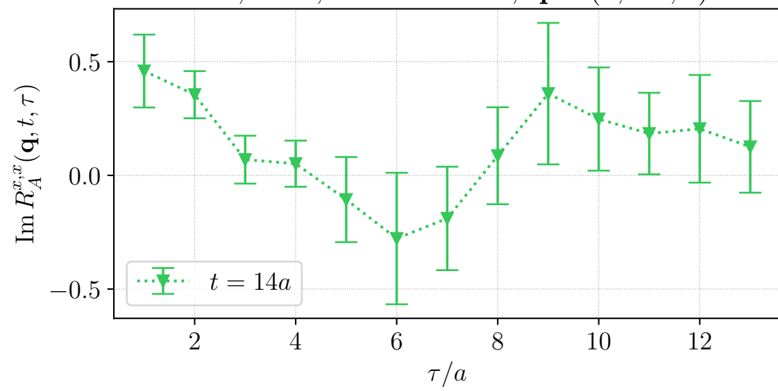
H106, LHP, source id = 1, \mathbf{q} \sim (0, -1, 2)^\top
