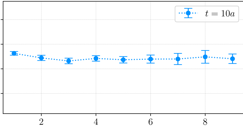
H106, REG, source id = 0, \mathbf{q} \sim (0, 1, -2)^\top
