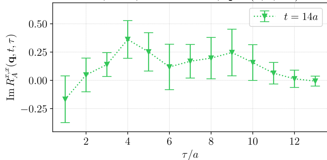
H106, LHP, source id = 1, \mathbf{q} \sim (0, 1, -2)^\top
