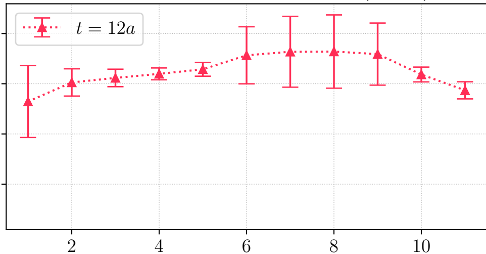
H106, REG, source id = 0, \mathbf{q} \sim (1, 1, 2)^\top
