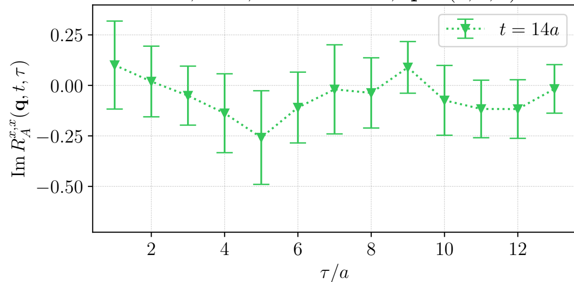
H106, LHP, source id = 1, \mathbf{q} \sim (1, 1, 2)^\top
