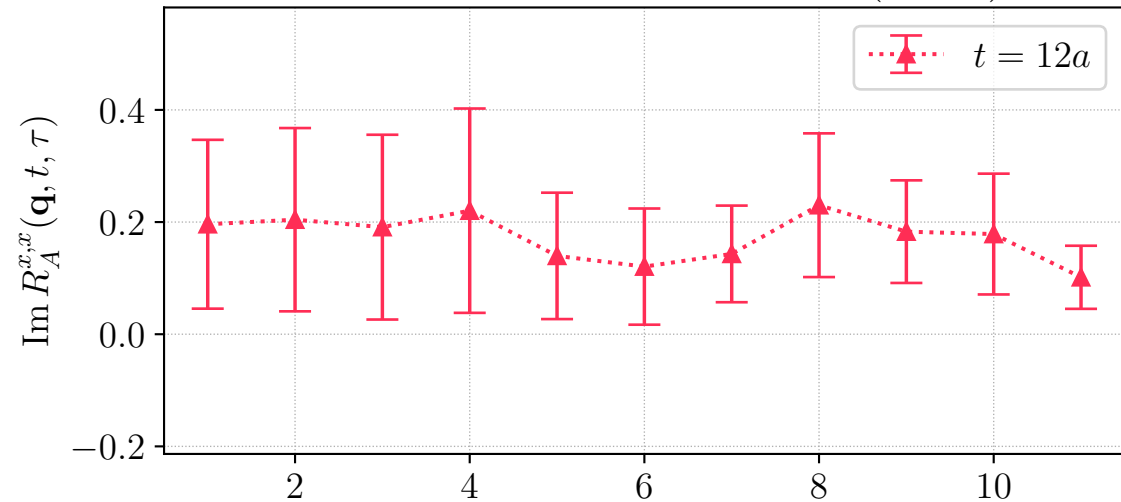
H106, LHP, source id = 0, \mathbf{q} \sim (2, 0, 1)^\top
