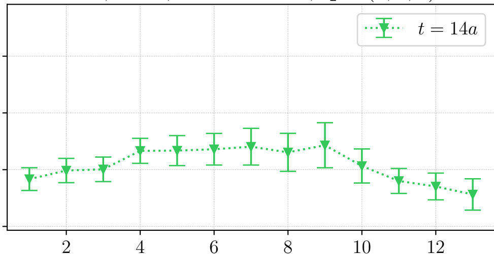
H106, REG, source id = 1, \mathbf{q} \sim (2, 0, 1)^\top
