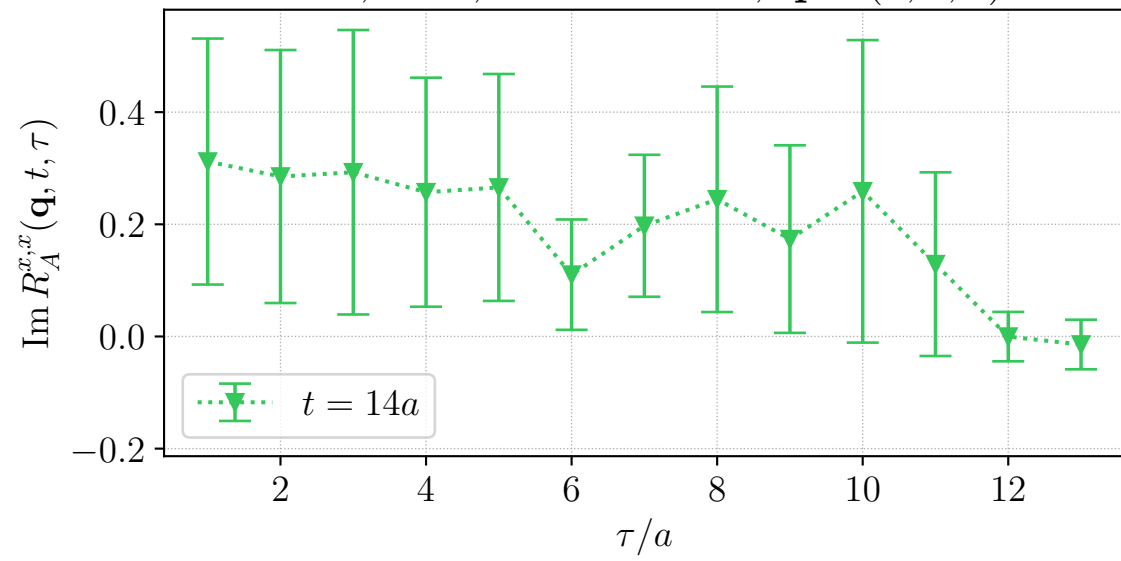
H106, LHP, source id = 1, \mathbf{q} \sim (2, 0, 1)^\top
