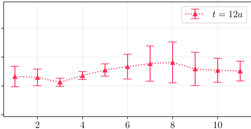
H106, REG, source id = 0, \mathbf{q} \sim (2, 0, 1)^\top
