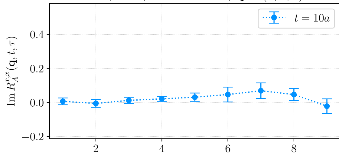
H106, LHP, source id = 1, \mathbf{q} \sim (2, 0, 1)^\top
