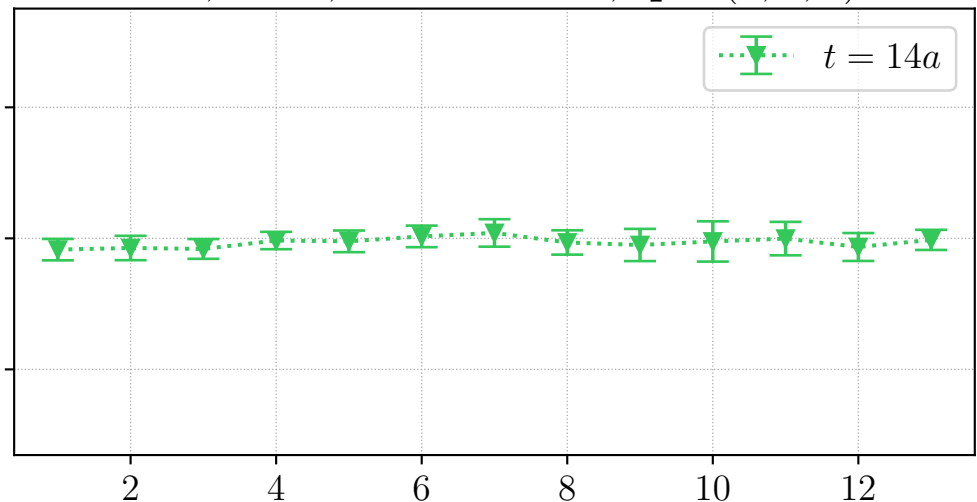
H106, REG, source id = 1, \mathbf{q} \sim (2, 2, 0)^\top
