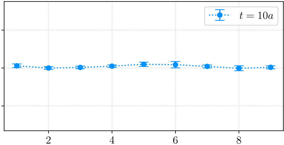
H106, REG, source id = 0, \mathbf{q} \sim (2, 2, 0)^\top
