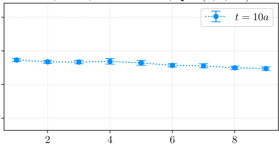
H106, REG, source id = 1, \mathbf{q} \sim (0, 1, -1)^\top
