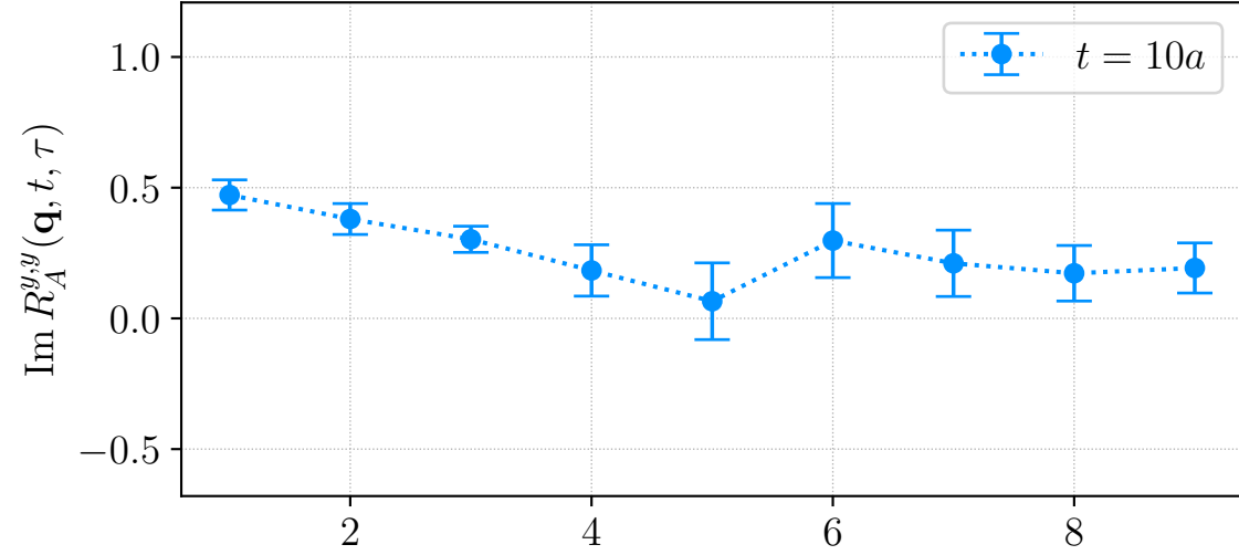
H106, LHP, source id = 0, \mathbf{q} \sim (0, 1, -1)^\top
