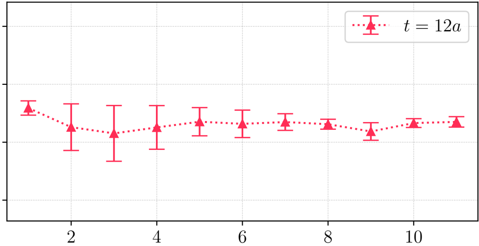
H106, REG, source id = 0, \mathbf{q} \sim (0, 1, -1)^\top
