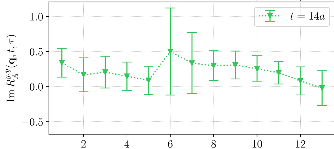
H106, LHP, source id = 1, \mathbf{q} \sim (0, 1, -1)^\top
