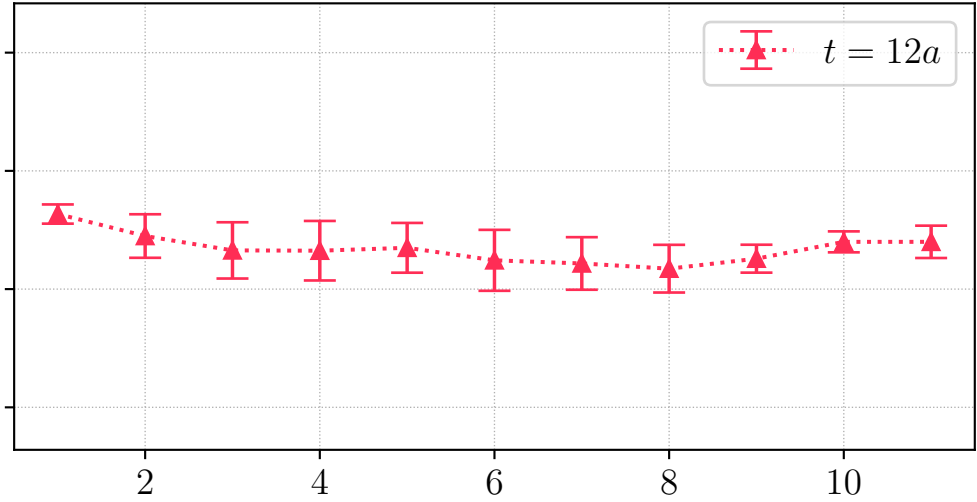
H106, REG, source id = 1, \mathbf{q} \sim (0, 1, -1)^\top
