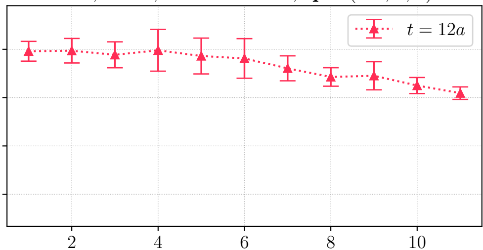
H106, REG, source id = 0, \mathbf{q} \sim (-1, 0, 0)^\top
