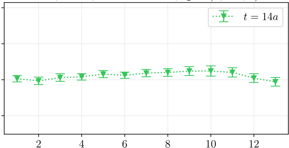
H106, REG, source id = 1, \mathbf{q} \sim (1, -2, 1)^\top
