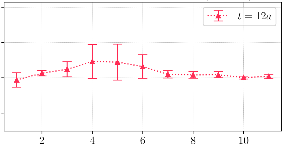
H106, REG, source id = 0, \mathbf{q} \sim (1, -2, 1)^\top
