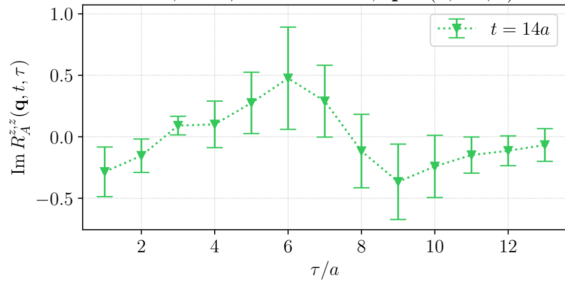
H106, LHP, source id = 1, \mathbf{q} \sim (1, -2, 1)^\top
