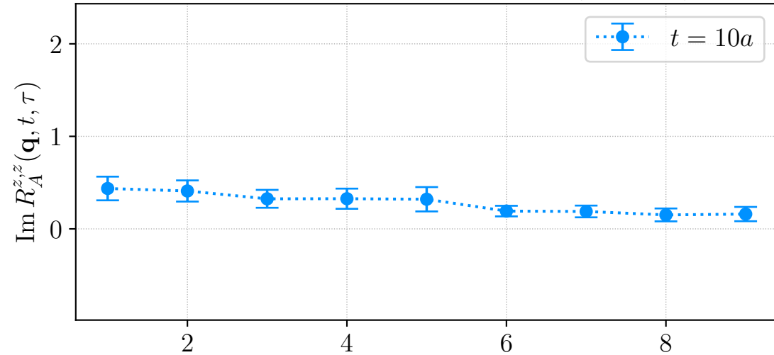
H106, LHP, source id = 0, \mathbf{q} \sim (1, 0, -1)^\top
