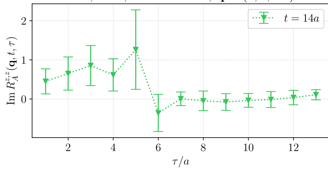
H106, LHP, source id = 1, \mathbf{q} \sim (1, 0, -1)^\top
