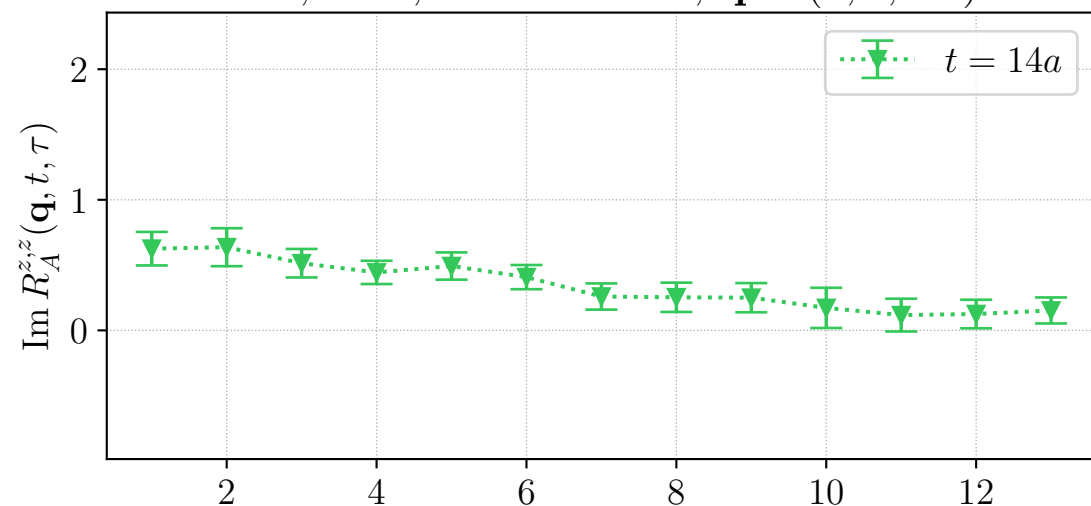
H106, LHP, source id = 1, \mathbf{q} \sim (1, 0, -1)^\top
