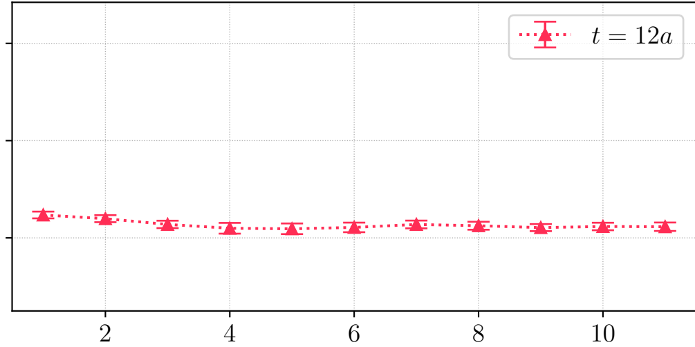
H106, REG, source id = 1, \mathbf{q} \sim (2, 0, 0)^\top
