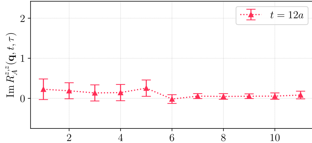
H106, LHP, source id = 0, \mathbf{q} \sim (2, 0, 0)^\top
