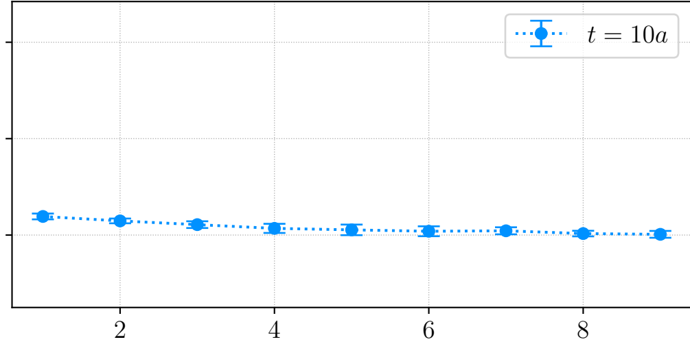
H106, REG, source id = 0, \mathbf{q} \sim (2, 0, 0)^\top
