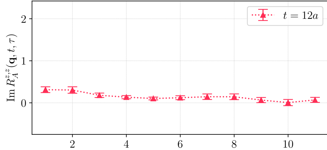
H106, LHP, source id = 1, \mathbf{q} \sim (2, 0, 0)^\top
