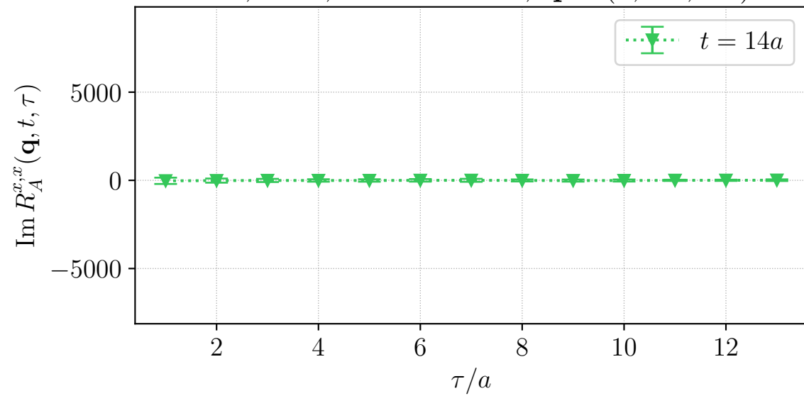
H107, LHP, source id = 1, \mathbf{q} \sim (1, -2, -1)^\top
