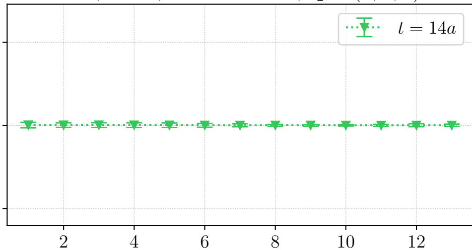
H107, REG, source id = 1, \mathbf{q} \sim (1, 2, 0)^\top
