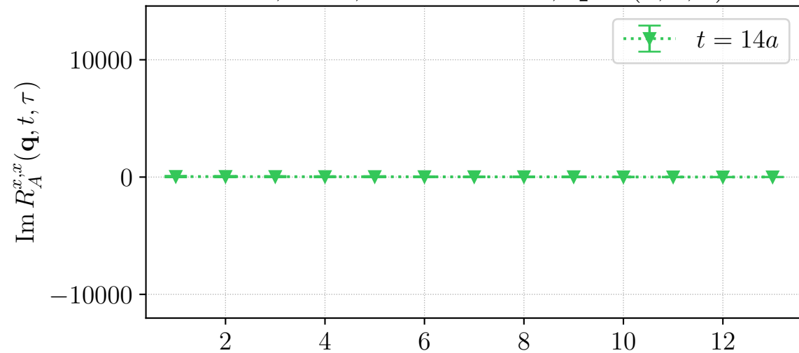
H107, LHP, source id = 1, \mathbf{q} \sim (1, 2, 0)^\top
