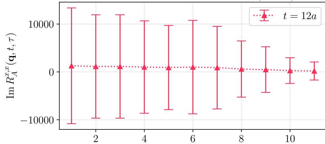
H107, LHP, source id = 0, \mathbf{q} \sim (1, 2, 0)^\top
