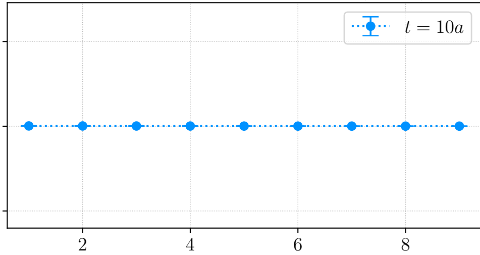
H107, REG, source id = 0, \mathbf{q} \sim (1, 2, 0)^\top
