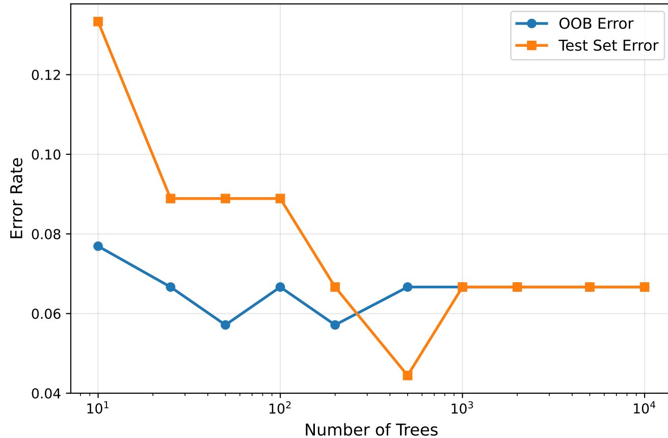
OOB Error vs Test Set Error Convergence
