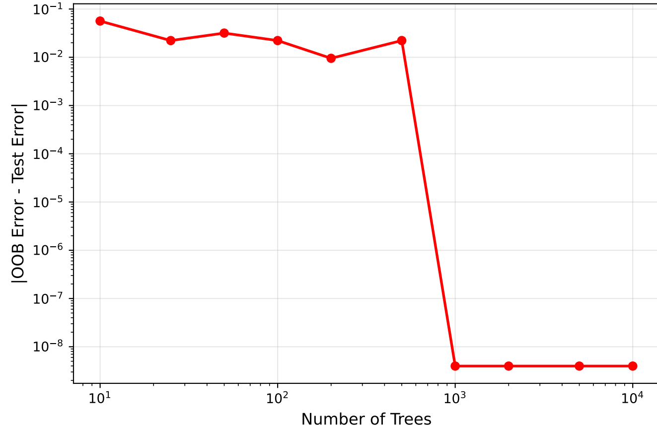
Convergence of OOB and Test Set Error
