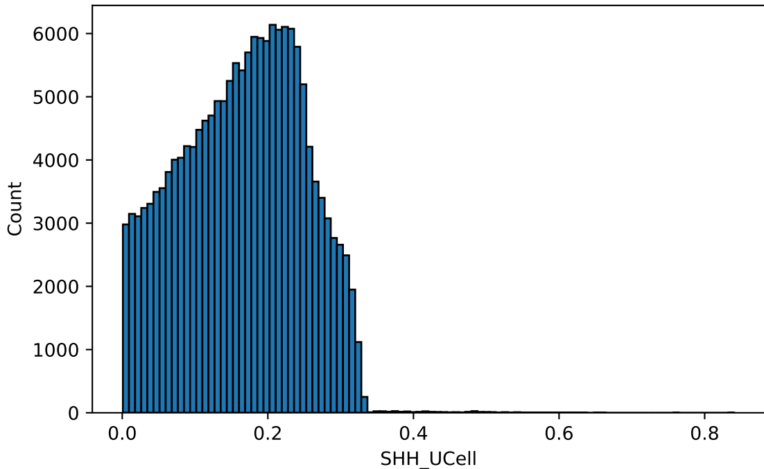
Blood ... All cells (no-zeros, n=167776)
