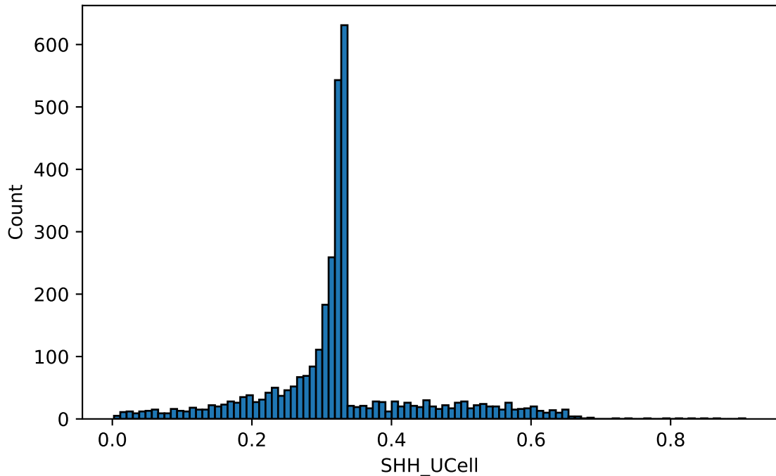
Notochord ... All cells (no-zeros, n=3320)
