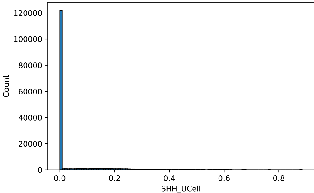
PNS_neurons ... All cells (all, n=146825, zero=82.7%)
