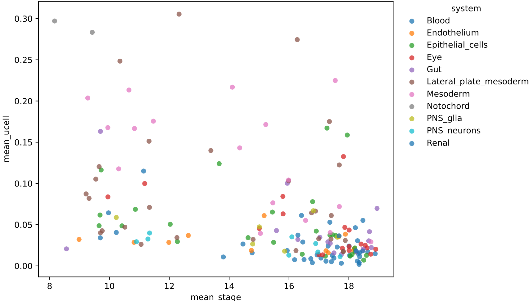
Mean UCell per node vs mean stage per node (colored by system)
