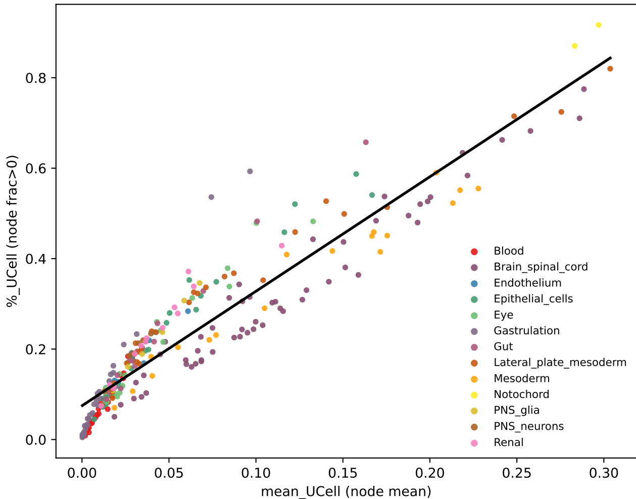
ALL systems node dots: mean_UCell vs %_UCell Spearman rho = 0.958
