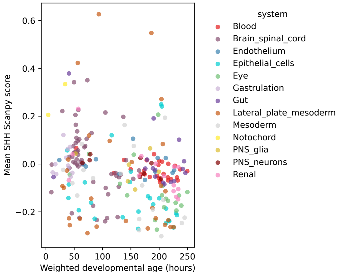
SHH Scanpy score vs developmental age
