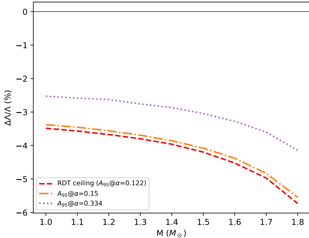
(b) Ceiling shift along the solar exclusion boundary
