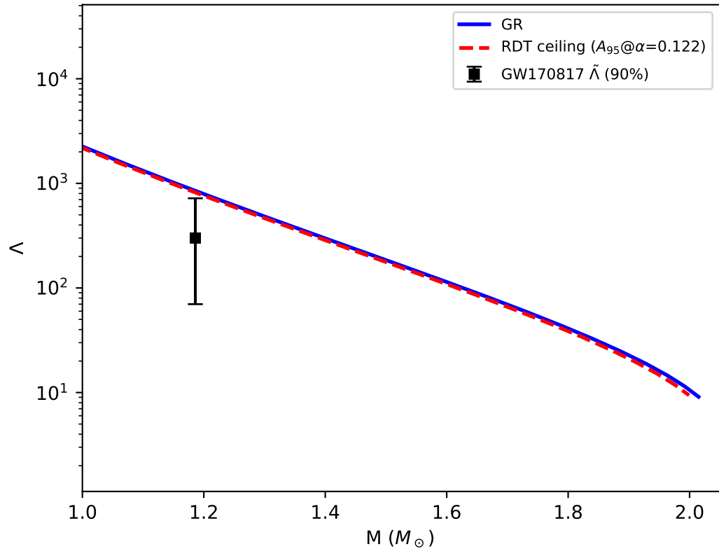
(a) Tidal deformability: GR vs maximum solar-allowed RDT
