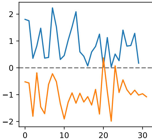
Session 1, CDdotprod -0.169
