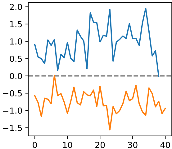
Session 1, CDdotprod -0.416
