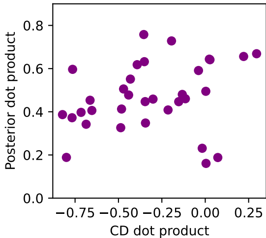
correlation 0.25
