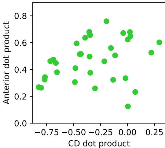
correlation 0.3
