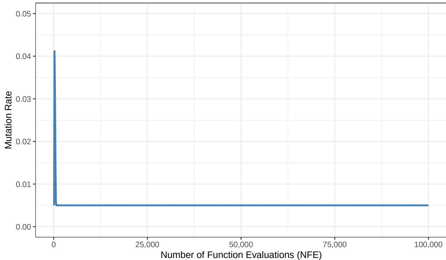
G06 – Adaptive Mutation Rate
